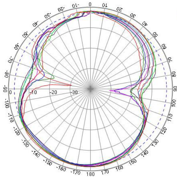
XY PLANE
