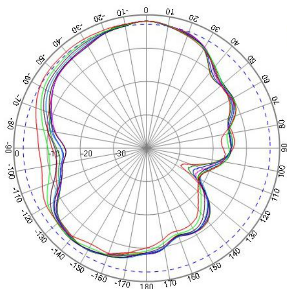
YZ PLANE
